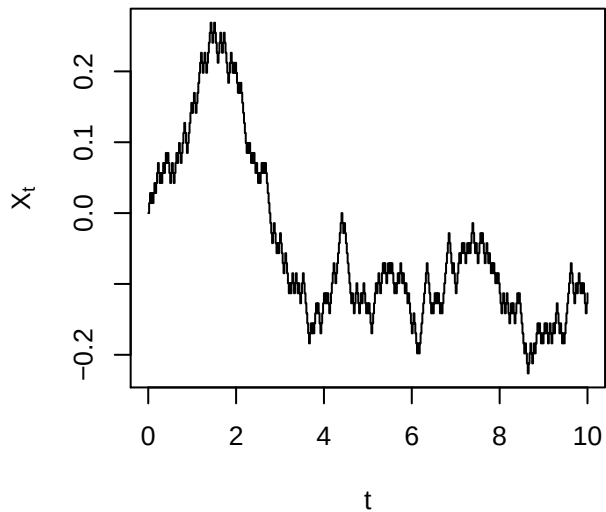
c = 50 sigma = 0.1
