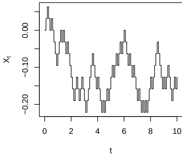
c = 10 sigma = 0.1
