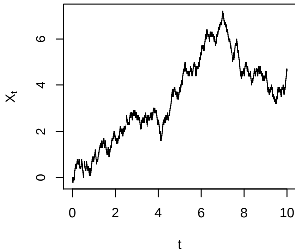
c = 100 sigma = 1
