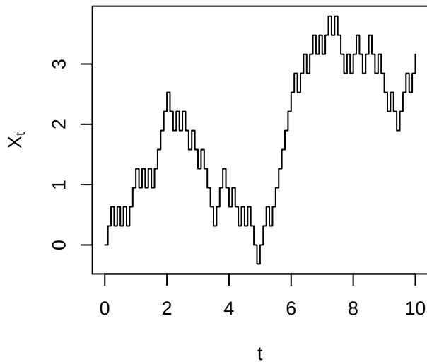
c = 10 sigma = 1
