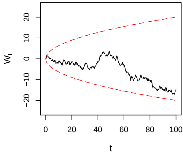
sigma = 1
