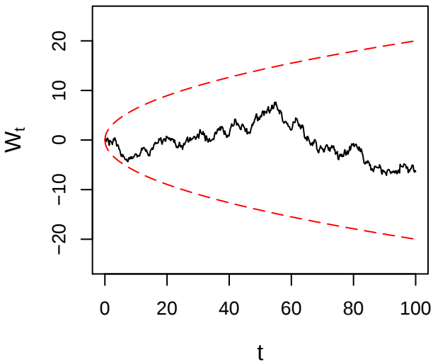
sigma = 1
