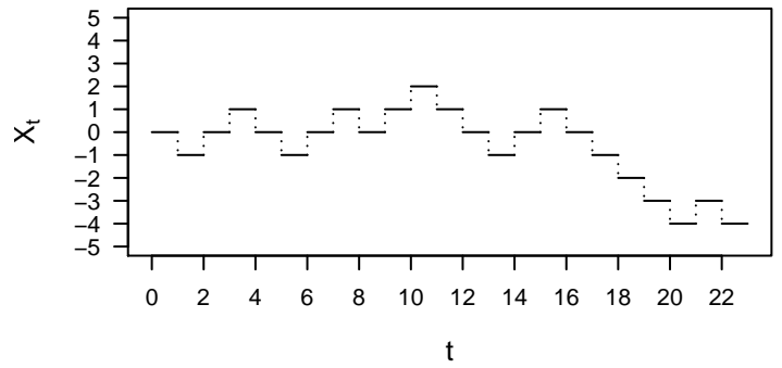
p = 0.5 q = 0.5 r = 0
