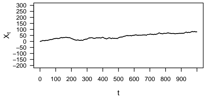
p = 0.51 q = 0.49 r = 0
