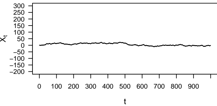
p = 0.49 q = 0.51 r = 0
