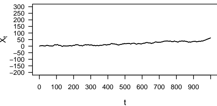
p = 0.5 q = 0.5 r = 0
