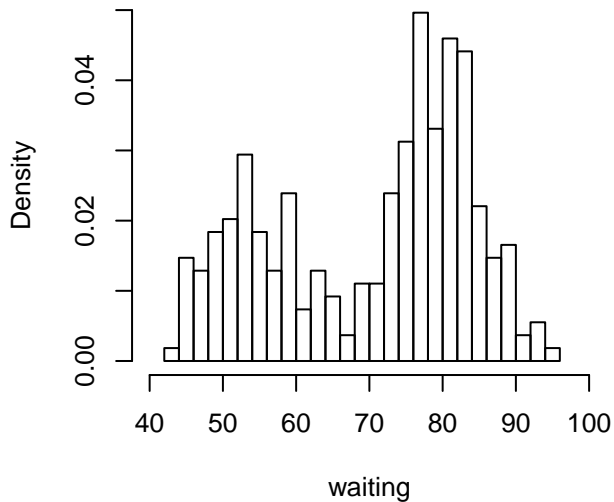
Histogramm: 'breaks = 20'
